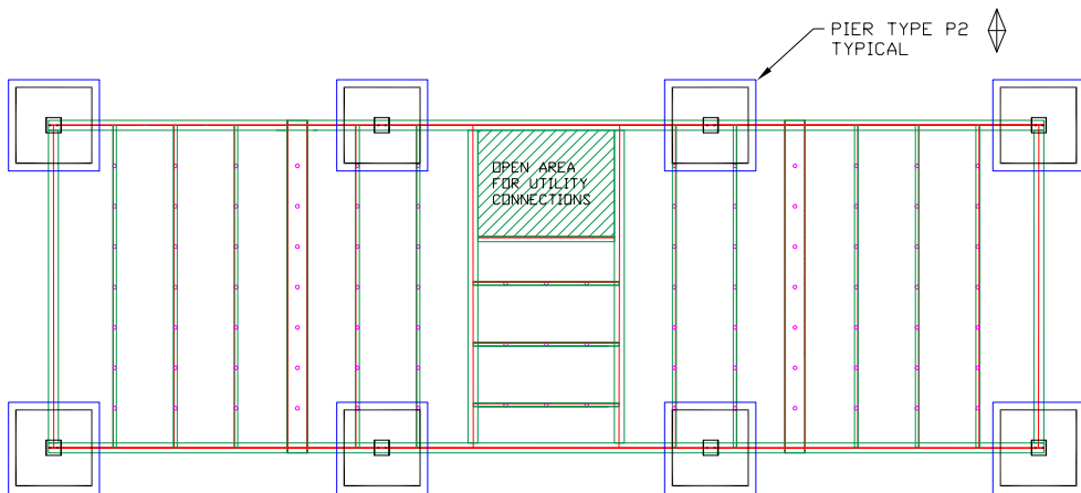
PIER LOCATION PLAN
