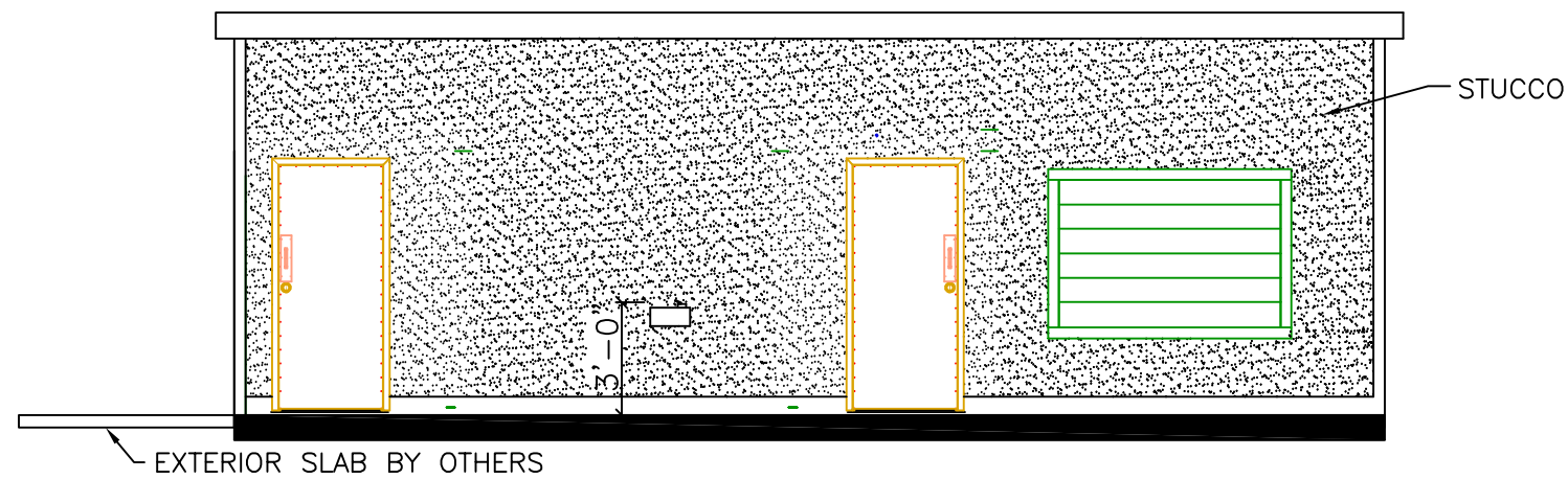
FRONT ELEVATION
