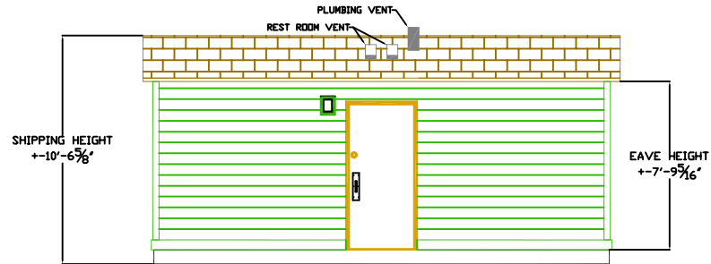
BACK ELEVATION
