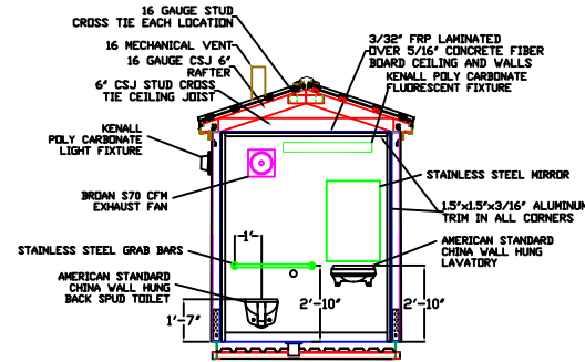
BUILDING SECTION VIEW LEFT SIDE
