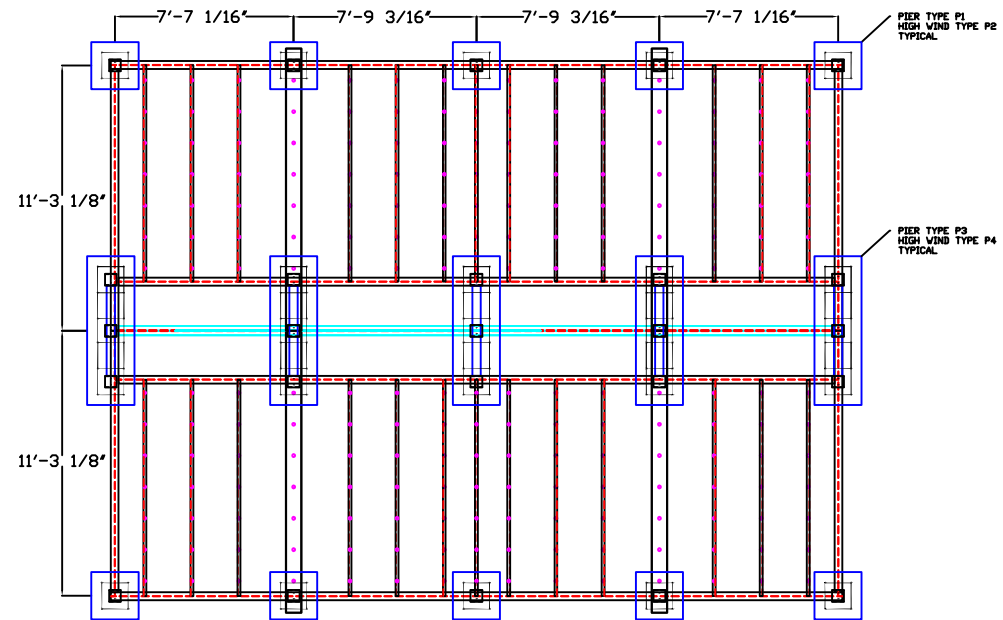
PIER LOCATION PLAN
