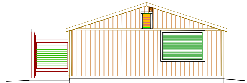
END ELEVATION @ CONCESSION WINDOW
