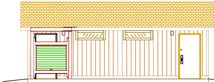
SIDE ELEVATION @ RESTROOM DOOR
