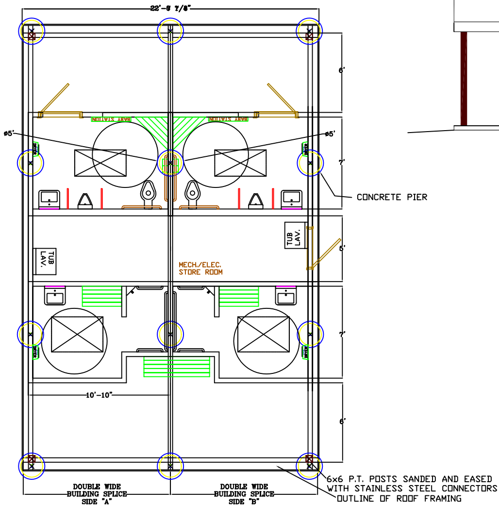
FLOOR PLAN
