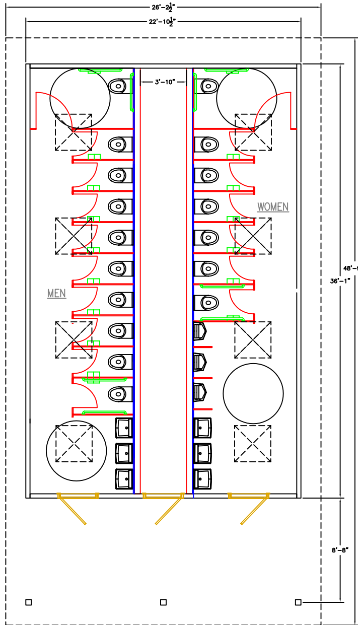
PLAN VIEW
